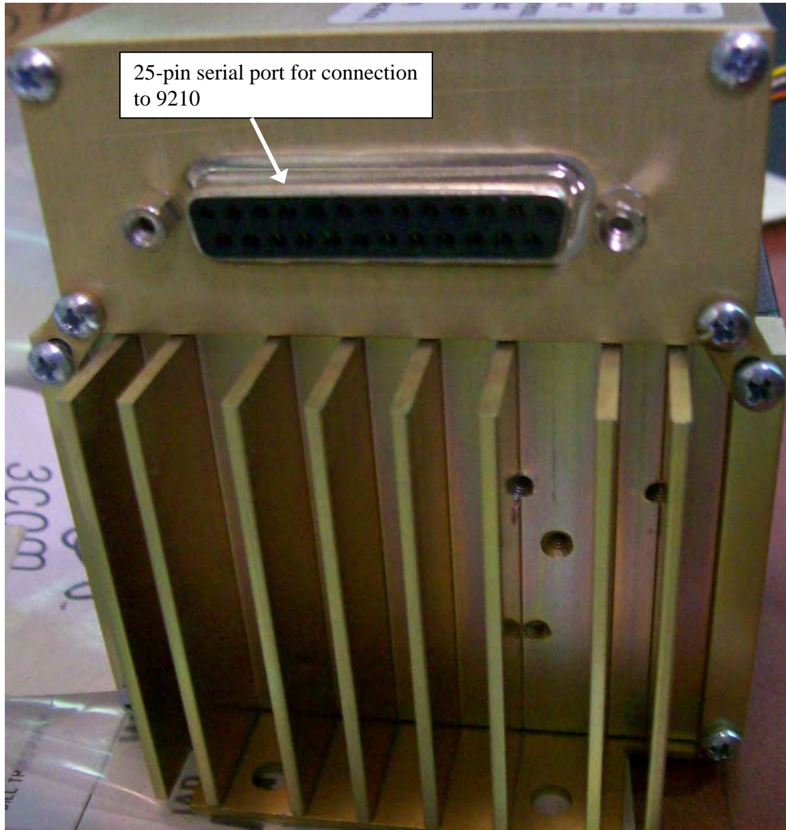
Figure 2: Back of DL3282 Modem showing 25-pin Serial Port
